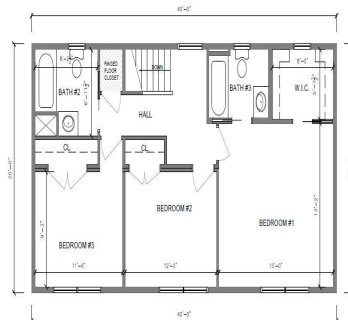
2ND FLOOR PLAN (#23036)
