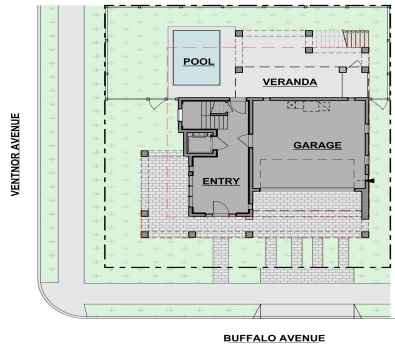
1 PLOT PLAN
